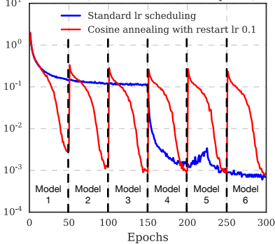
Cifar10 (L=100,k=24, B=300 epochs)
